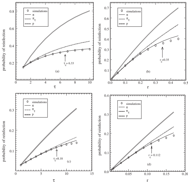
FIG. 2. Simulation and theory for the reinfection probability. Three approximations, p (dot-dashed lines), \pi_t (dashed lines), \pi (solid lines), are compared with simulation results (see text). Simulation results (circles) were obtained by recording the probability of an infected node to reinfect its ancestors, averaging over many network and disease configurations. The simulations presented are for ER networks but were validated also for SF networks. The epidemic threshold is indicated with an arrow, and is calculated from Eq. (7). (a) \kappa = 2.1 , r = 0.15 , and increasing values of \tau ; (b) \kappa = 2.1 , \tau = 2 , and increasing values of r ; (c) \kappa = 5 and r = 0.03 ; (d) \kappa = 5 and \tau = 2 .
