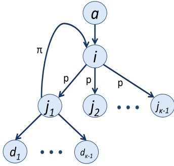
FIG. 1 (color online). A schematic illustration of the subnetwork in which the probabilities of infections are calculated in the text.
