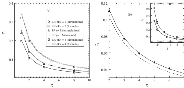
FIG. 3. Simulation results for the critical infection rate. (a) Simulation results of r_c vs \tau for ER networks with \langle k \rangle = 2, 4 and SF networks with \gamma = 3.6 (symbols), compared to theory (lines) as obtained from Eq. (7). (b) Theoretical values of r_c [Eq. (7), solid line] compared to the mean-field approach [obtained by setting \pi = p in Eq. (7), dashed line] and simulation (circles) for \langle k \rangle = 4 . The inset compares r_c (theory and simulations) between SIR (circles) and SIS (squares) with \langle k \rangle = 2 . Theoretical values (lines) were obtained from Eq. (3) for SIR and from Eq. (7) for SIS. The epidemic threshold was calculated using a method of percolation theory: we denote by S the total number of infections; r_c was identified as r for which S \sim N [19,20].
