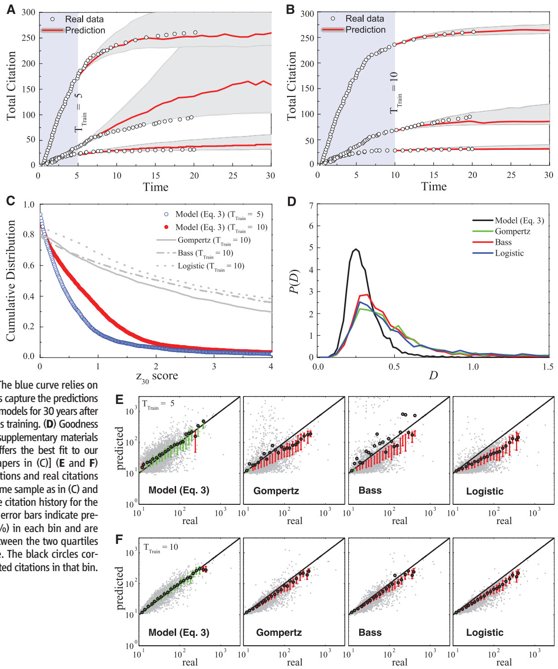
Fig. 4. Predicting future citations.
