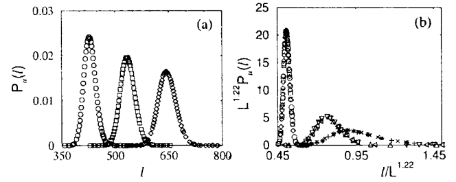
FIG. 2. (a) Plot of P(\ell|L,u) vs \ell for square lattices with fixed u \equiv L/a^\nu = 10 and different values of L . (b) Plot of P(\ell|L,u)L^{1.22} vs \ell/L^{1.22} . Three families of curves are shown and each family has the same ratio u \equiv L/a^\nu : u=10 [ L=250 ( \circ ), L=300 ( \square ), L=350 ( \diamond )]; u=1.26 [ L=30 ( \triangle ), L=40 ( \triangleleft ), L=60 ( \nabla )]; u=0.25 [ L=15 ( + ), L=20 ( \times ), L=27 ( * )]. The distribution curves with the same ratio of u collapse both in weak disorder such as u=10 and in strong disorder such as u=0.25 , as well as in the intermediate regime u=1.26 for a > 10 and L > 15 . We compute all the data with 1000 realizations of disorder and 10^5 tracers for each realization.
