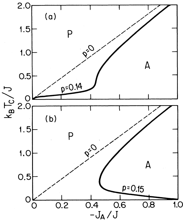
FIG. 2. The exact phase diagram of the 2D decorated Ising model for different values of the concentration p of decorated bonds. The transition line for (a) p=0.14 ( p < p_c ) and (b) p=0.15 ( p > p_c ) illustrates the drastic transition from one regime to another. Here A and P denote the antiferromagnetic and the paramagnetic regions, respectively, and the exact frontier between A and P for p=0 is also shown.
