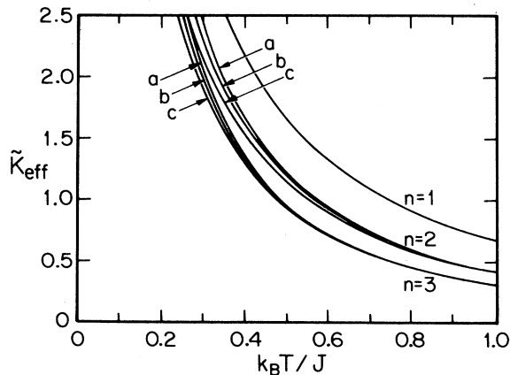
FIG. 1. The decorated effective coupling \tilde{K}_{\text{eff}} as a function of the reduced temperature k_B T/J for the Ising ( n=1 ), XY ( n=2 ), and Heisenberg ( n=3 ). The curves labeled (a), (b), and (c), are for \theta=0 , \theta=\pi/6 , and \theta=2\pi/3 , respectively.
