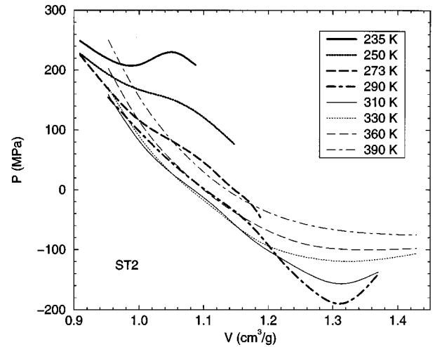
FIG. 2. Equation of state of liquid ST2. Plotted are isotherms of P versus V of a cubic spline through the data points tabulated in Ref. [20], from T=235 K to T=390 K.
