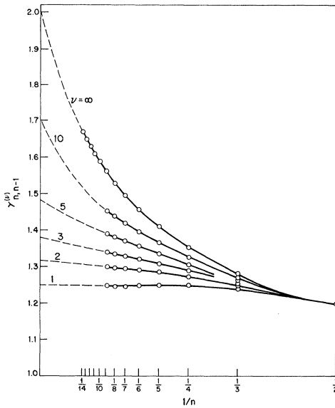
FIG. 2. Variation of \gamma(\nu) with \nu for the fcc lattice. The function \gamma_{n,n-1}(\nu) \equiv 1 - n + n\rho_n(\nu)/t_{n,n-1}(\nu) , where t_{n,n-1}(\nu) \equiv n\rho_n(\nu) - (n-1)\rho_{n-1}(\nu) , gives the value of \gamma which would be obtained by placing a straight line through the ratios \rho_n(\nu) and \rho_{n-1}(\nu) (plotted against 1/n as, e.g., in Fig. 1). Thus \gamma_{n,n-1}(\nu) should approach \gamma(\nu) as n \rightarrow \infty if \chi diverges with a power law as T \rightarrow T_c(\nu) . One of the extrapolations shown is exact: \gamma(\infty) = 2 . Curves for other values of \nu lie between the ones shown.
