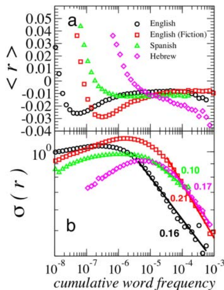
Figure 7 | Scaling in the growth rate fluctuations of words. We show the dependence of growth rates on the cumulative word frequency S_i \equiv \sum_{\tau=0}^i f_i(\tau) using words satisfy the criteria T_i \geq 10 years. We verify similar results for threshold values T_c = 50, 100, and 200 years. (a) Average growth rate \langle r \rangle saturates at relatively constant values for large S . (b) Scaling in the standard deviation of growth rates \sigma(r|S) \sim S^{-\beta} for words with large S . This scaling relation is also observed for the growth rates of large economic institutions, ranging in size from companies to entire countries 31,33 . Here this size-variance relation corresponds to scaling exponent values 0.10 < \beta < 0.21 , which are related to the non-trivial bursting patterns and non-trivial correlation patterns in literature topicality as indicated by the quantitative relation to the Hurst exponent, H = 1 - \beta shown in 35 . We calculate \beta_{Eng.} \approx 0.16 \pm 0.01 , \beta_{Eng.fict} \approx 0.21 \pm 0.01 , \beta_{Spa.} \approx 0.10 \pm 0.01 and \beta_{Heb.} \approx 0.17 \pm 0.01 .
