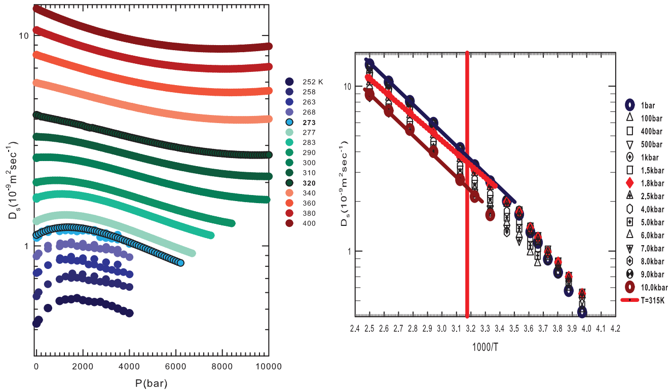
Figure 4 | (a) The bulk water self-diffusion coefficient D_S as a function of the pressure in the range 1 \text{ bar} < P < 10 \text{ kbar} at different temperatures from the supercooled region 252 \text{ K} to 400 \text{ K} . (b) The self-Diffusion coefficient D_S , at several different pressures from 1 \text{ bar} to 10 \text{ kbar} in an Arrhenius fit ( \log D_S vs 1000/T ). The red line represents the T^* temperature crossover that identifies two different scenarios, Arrhenius for T > T^* and super-Arrhenius for T < T^* . I.e. the transition of water from a simple to a strong interacting structured liquid.
