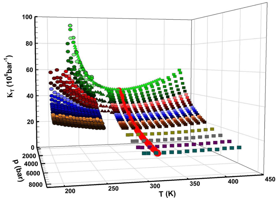
Figure 2 | The bulk water isothermal compressibility K_T(T, P) in the same P, T ranges of the density data illustrated in the Figure 1, the pressures are identified by means of the same symbols 16,18,19,23,25–27 . A simple data inspection shows: i) two distinct behaviors of the K_T dependence, at the different pressures, in the high and low temperature regimes; ii) at all the reported pressures the K_T(T) curves present a minimum value located at the same temperature T^* \sim 315 \text{ K} \pm 5 \text{ K} ; iii) also for K_T , like for \rho , it seems that P_{\text{cross}} is at the borderline of two regions; one of very large volume fluctuations ( P < P_{\text{cross}} ) and a second one where \langle \delta V^2 \rangle is comparable with that of the liquid in its stable phases.
