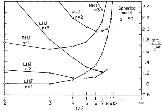
FIG. 7. Spherical model \bar{\chi}^{\text{sc}} series sequences for \phi T_c/T_c^{\text{MF}} given by Eq. (4.10). These curves all bend upward and eventually begin to oscillate.
