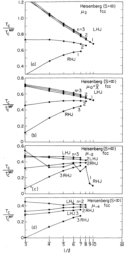
FIG. 6. Sequence of Eq. (4.11) for the classical Heisenberg model fcc lattice series are shown for the spherical moments t=2, 0, -2 , and -4 in parts (a), (b), (c), and (d), respectively. The points for the n=1, t=-4 sequence are oscillatory, as expected, and are therefore not shown. Values of these for l=3-10 are 0.734, 0.133, 0.012, 0.252, -21.019 , 0.229, 1.065, and 0.221.
