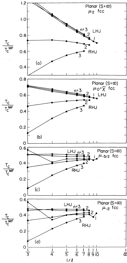
FIG. 5. Sequences of Eq. (4.11) for the classical planar model fcc lattice series are shown for the spherical moments, Eq. (1.1), t=2, 0, -\frac{3}{2} , and -2 in parts (a), (b), (c), and (d), respectively. The notation LHJ and RHJ is explained in the text.
