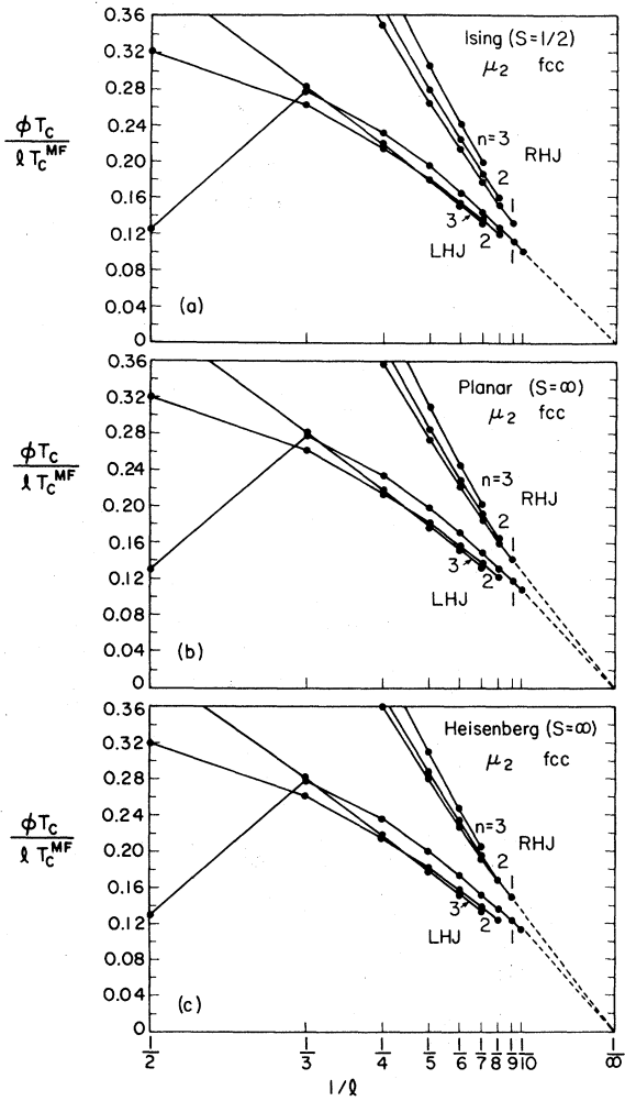
FIG. 2. Sequences shown are given by Eq. (4.9) and should converge to the origin with slope \phi T_c/T_c^{MF} . The series used are \mu_2^{fcc} for the (a) Ising, (b) planar, and (c) classical Heisenberg models. The dashed line on the Ising model plots uses the known exact results while the lines on the other models are visual guides only.
