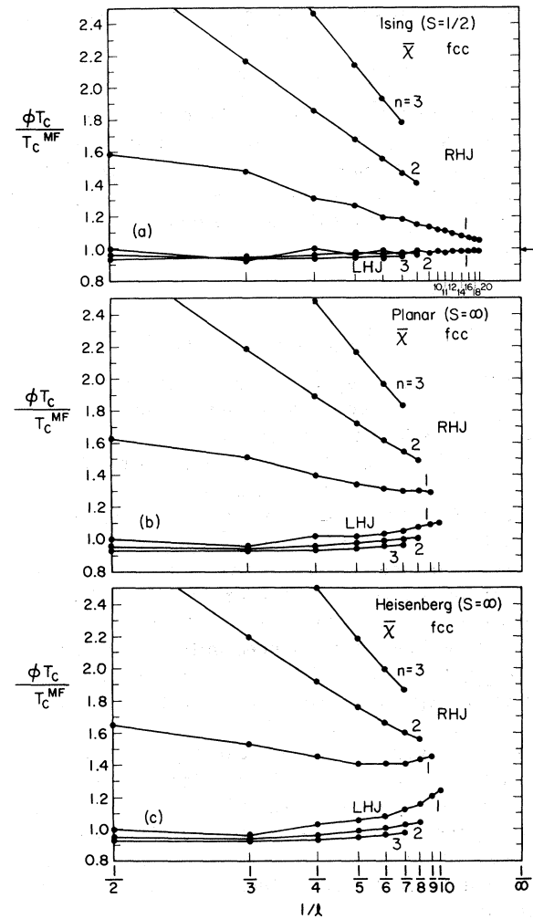
FIG. 3. These curves represent quantities defined by Eq. (4.10) and should converge to the product \phi T_c/T_c^{MF} . Part (a) uses the Ising model \bar{\chi}^{fcc} series while (b) and (c) are the planar and Heisenberg models.
