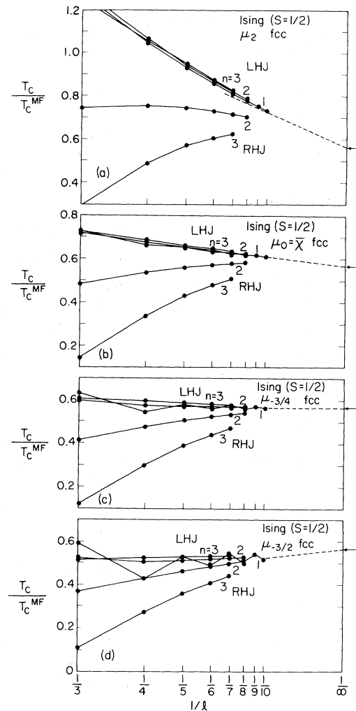
FIG. 4. Sequences of Eq. (4.11) for the Ising model fcc lattice series are shown for the spherical moments [Eq. (1.1)] with t=2, 0, -\frac{3}{4} , and -\frac{3}{2} in parts (a), (b), (c), and (d), respectively. The notation LHJ and RHJ refers to how the ratios are plotted and is explained in the text.
