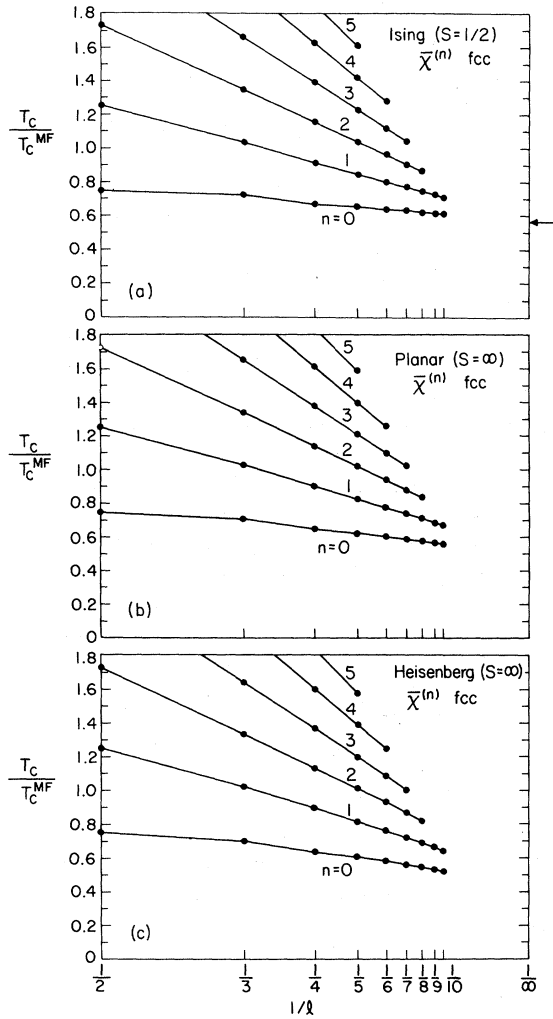
FIG. 1. Series ratios defined in Eq. (4.6) are plotted for \bar{\chi}^{\text{fcc}} for the (a) Ising, (b) planar, and (c) classical Heisenberg models (see Ref. 14). The arrow indicates the exact value for D=1 .
