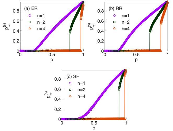
FIG. 2. The percolation behaviors of treelike networks of (a) ER networks ( \langle k \rangle = 10 ), (b) RR networks ( \langle k \rangle = 10 ), and (c) SF networks ( \lambda = 2.5 ). For a single network ( n = 1 ), the size of the final GSCC continuously decreases to zero when the fraction of remaining nodes p decreases. When the system composes more than two networks ( n \geq 2 ), the size of the final GSCC discontinuously jumps to zero at a critical point p_c^1 . The symbols represent simulation results (each network layer contains N = 10^6 nodes), the solid lines are theoretic results, and they agree well with each other.
