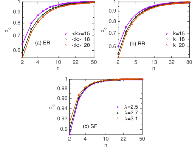
FIG. 4. The critical point p_c^1 of treelike networks of n (a) ER networks with different average degrees \langle k \rangle , (b) RR networks with different degrees k , and (c) SF networks with different degree distribution exponents \lambda . The results of the ER networks and the RR network are computed by Eqs. (28) and (34), respectively. The results of the SF networks are computed by substituting Eq. (37) with Eq. (17). They are in good agreement with simulations. As more networks are added in, the critical point p_c^1 increase, indicating the more vulnerable the system is.
