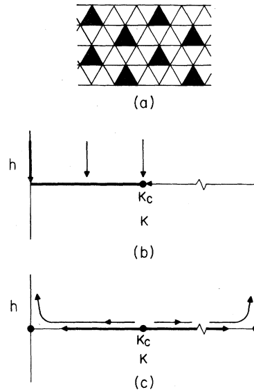
FIG. 1. (a) Triangular lattice with three-spin cells. (b) Phase diagram indicating the percolation transitions on a two-dimensional triangular lattice. The line 0 \leq K \leq K_c is a line of percolation points. The arrows indicate the paths along which the percolation points are approached. (c) Schematic diagram illustrating RG flow lines in the h - K plane. At h=0 , for K < K_c , the flow is to the K=0 fixed point, while for K > K_c , the flow is to the K=\infty fixed point, and at K=K_c , the flow, in the higher-dimensional coupling-constant space (not shown), is to the Ising fixed point.
