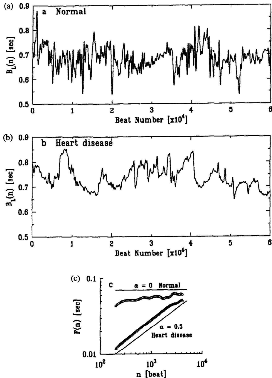
Fig. 13. The interbeat interval B_L(n) after low-pass filtering for (a) a healthy subject and (b) a patient with severe cardiac disease (dilated cardiomyopathy). The healthy heartbeat time series shows more complex fluctuations compared to the diseased heart rate fluctuation pattern that is close to random walk ("brown") noise. (c) Log-log plot of F(n) vs n . The circles represent F(n) calculated from data in (a) and the triangles from data in (b). The two best-fit lines have slope \alpha = 0.07 and \alpha = 0.49 (fit from 200 to 4000 beats). The two lines with slopes \alpha = 0 and \alpha = 0.5 correspond to "1/f noise" and "brown noise," respectively. We observe that F(n) saturates for large n (of the order of 5000 beats), because the heartbeat intervals are subjected to physiological constraints that cannot be arbitrarily large or small. The low-pass filter removes all Fourier components for f \geq f_c . The results shown here correspond to f_c = 0.005 \text{ beat}^{-1} , but similar findings are obtained for other choices of f_c \leq 0.005 . This cut-off frequency f_c is selected to remove components of heart rate variability associated with physiologic respiration or pathologic Cheyne-Stokes breathing as well as oscillations associated with baroreflex activation (Mayer waves). After [88]
