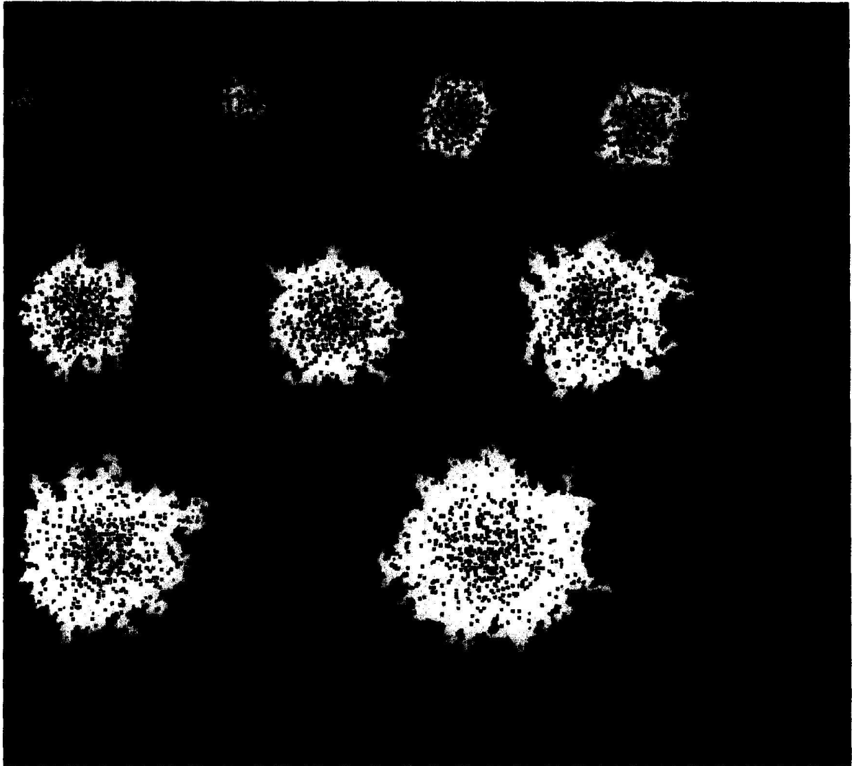
Fig. 5. Snapshots at successive times of the territory covered by N random walkers for the case N = 500 for a sequence of times. Note the roughening of the disc surface as time increases. The roughening is characteristic of the experimental findings for the diffusive spread of a population [21]. After [20], courtesy of P. Trunfio
