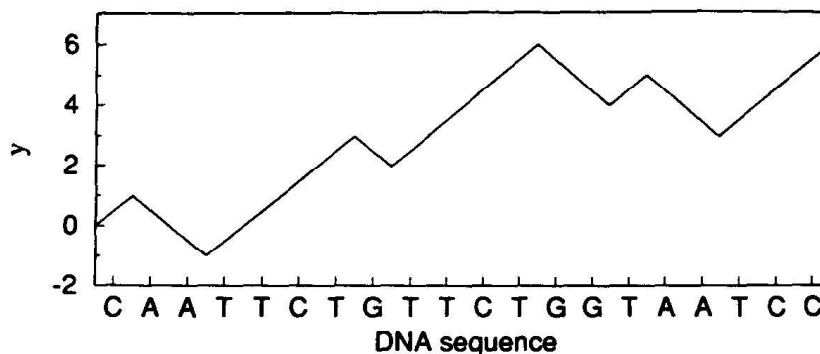
Fig. 7. Schematic illustration showing the definition of the “DNA walk”
