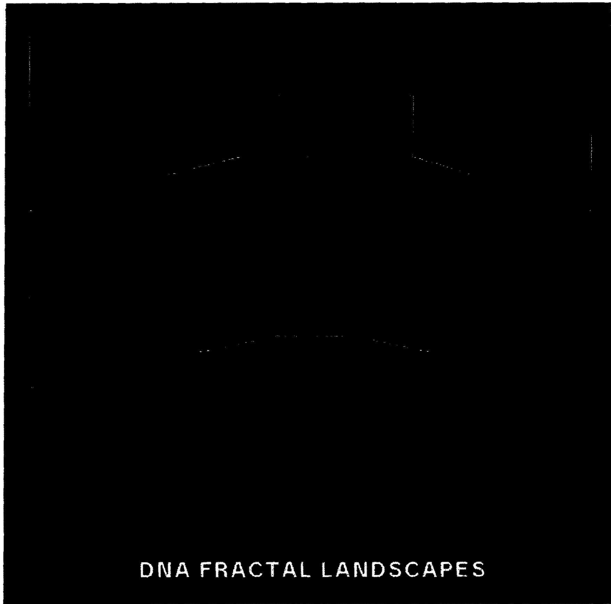
Fig. 11. The DNA walk representation for the rat embryonic skeletal myosin heavy chain gene ( \alpha = 0.63 ). At the top the entire sequence is shown. In the middle the solid box shown in the top is magnified. At the bottom the solid box shown in the middle is magnified. The statistical self-similarity of these plots is consistent with the existence of a scale-free or fractal phenomenon which we call a fractal landscape. Note that one must magnify the segment by different factors along the \ell (horizontal) direction and the y (vertical) direction; since F has the same units (dimension) as y , these magnification factors M_\ell and M_y (along \ell and y directions respectively) are related to the scaling exponent \alpha by the simple relation \alpha = \log(M_y)/\log(M_\ell) [e.g., from top to middle, \log(M_y)/\log(M_\ell) = \log(2.07)/\log(3.2) = 0.63 ]
