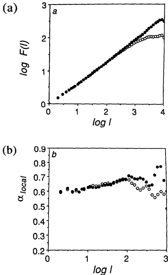
Fig. 9. (a) Double logarithmic plots of the mean square fluctuation function F(\ell) as a function of the linear distance \ell along the DNA chain for the rat embryonic skeletal myosin heavy chain gene ( \circ ) and its “intron-spliced sequence” ( \bullet ). (b) The corresponding local slopes, \alpha_{\text{local}} , based on pairs of successive data points of part (a). We see that the values of \alpha are roughly constant. For this specific gene, the sequence with exons removed has an even broader scaling regime than the DNA sequence of the entire gene, indicated by the fact that part (a) is linear up to 10,000 nucleotides. After [42]
