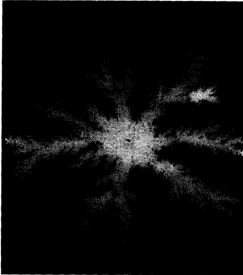
Fig. 4. A typical example of DLA-like colony patterns incubated at 35^{\circ}\text{C} for three weeks after inoculation on the surface of agar plates containing initially 1\text{ g/l} of peptone as nutrient. This pattern has a fractal dimension of \{d_f \cong 1.72\}^2 . After Matsushita and Fujikawa [16]
