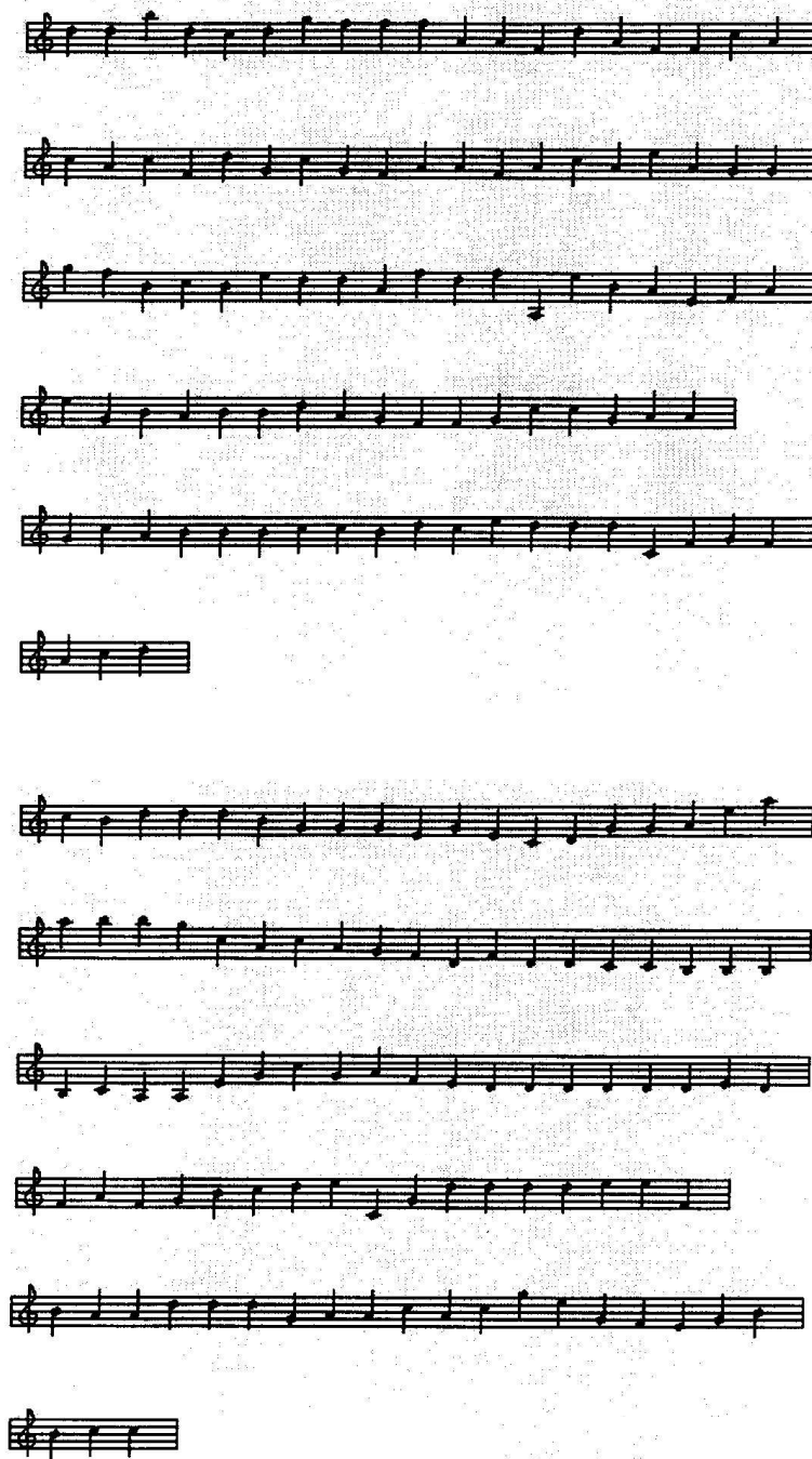
Fig. 15. Musical mapping of two heartbeat times series, derived from normal (top) and pathologic (bottom) data sets. The original heart beat time series were obtained from 24 hour recordings consisting of about 10^6 heartbeats. The heartbeat time series were then low-pass filtered to remove fluctuations > 0.05 ( \text{beat}^{-1} ), roughly equivalent to averaging every 200 beats. The pattern of fluctuations in the normal is more complex than that of the “music” generated from the abnormal data sets. Musical compositions based on these times series are available on cassette by request along with the “scores”; contact Zachary D. Goldberger (e-mail: ary “at” astro.bih.harvard.edu). There is a nominal charge for copying and mailing. After [97], courtesy of Z.D. Goldberger
