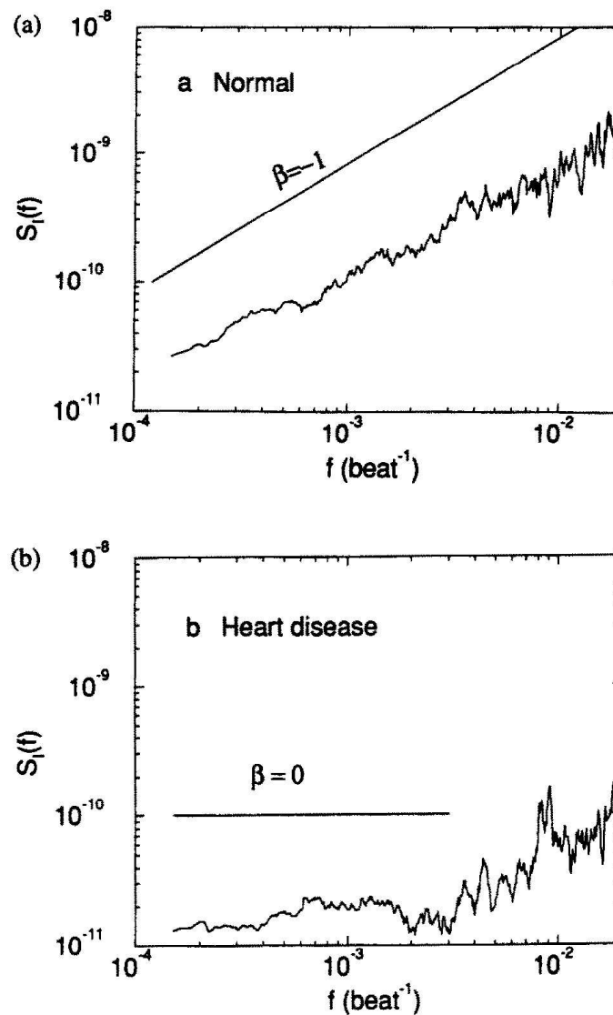
Fig. 14. The power spectrum S_I(f) for the interbeat interval increment sequences over \sim 24 hours for the same subjects in Fig. 13. (a) Data from a healthy adult. The best-fit line for the low frequency region has a slope \beta = -0.93 . The heart rate spectrum is plotted as a function of “inverse beat number” ( \text{beat}^{-1} ) rather than frequency ( \text{time}^{-1} ) to obviate the need to interpolate data points. The spectral data are smoothed by averaging over 50 values. (b) Data from a patient with severe heart failure. The best-fit line has slope 0.14 for the low frequency region, f < f_c = 0.005 \text{ beat}^{-1} . The appearance of a pathologic, characteristic time scale is associated with a spectral peak (arrow) at about 10^{-2} \text{ beat}^{-1} (corresponding to Cheyne-Stokes respiration). After [88]
